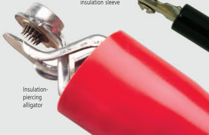
Standard alligator with insulation sleeve
