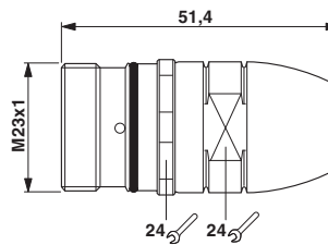
Dimensioned drawing
