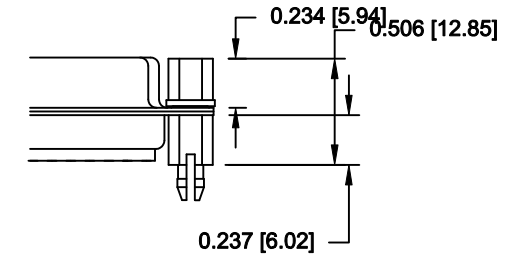
91X ..... 0.237" BOARD SIDE 0.197 MATING SIDE CN10/SFSO4404
