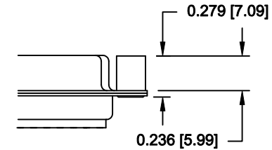
03X..... 0.236" (MATING SIDE) - CN8
