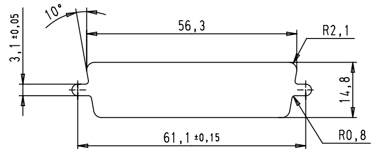
Panel cut out
