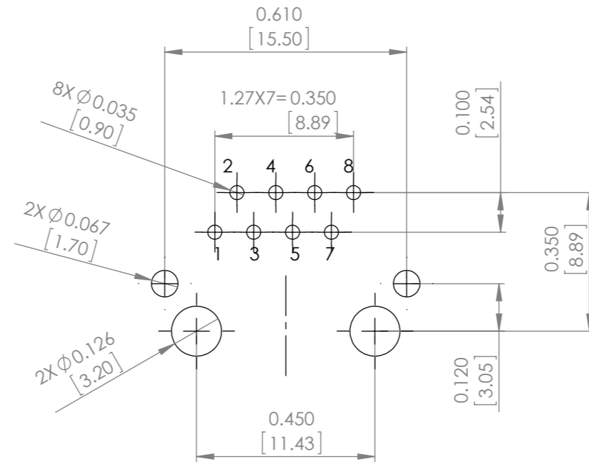
PC BOARD LAYOUT COMPONENT SIDE SHOWN
